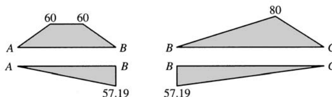
(g) Bending Moment Diagrams for Members AB and BC (k-ft)
