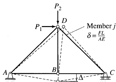
(a) Real System
