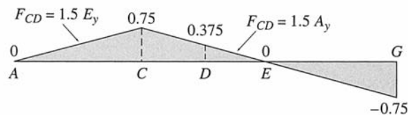
(g) Influence Line for F_{CD} (k/k)
