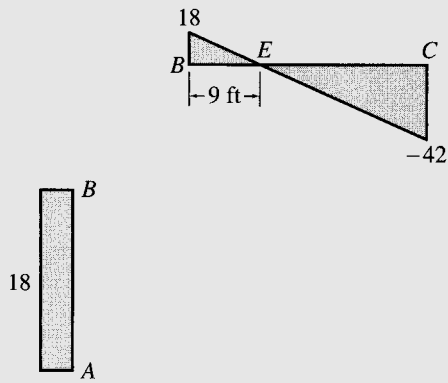
(e) Shear Diagrams (k)
