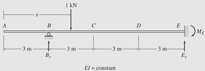
(a) Indeterminate Beam
