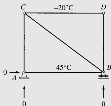
(b) Primary Truss Subjected to Temperature Changes
