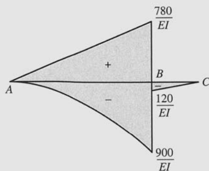
(b) \frac{M}{EI} Diagram ( \frac{\text{k}\cdot\text{ft}}{EI} )
