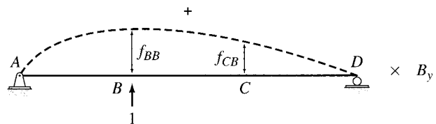
(c) Primary Beam Loaded with Redundant B_y
