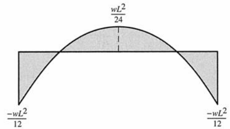
Bending Moment Diagram
