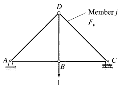
(b) Virtual System
