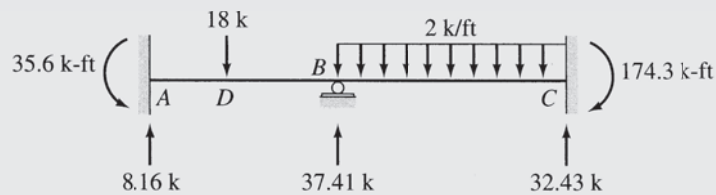
(c) Member End Moments and Shears
