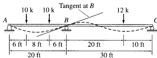
(a) Indeterminate Beam
