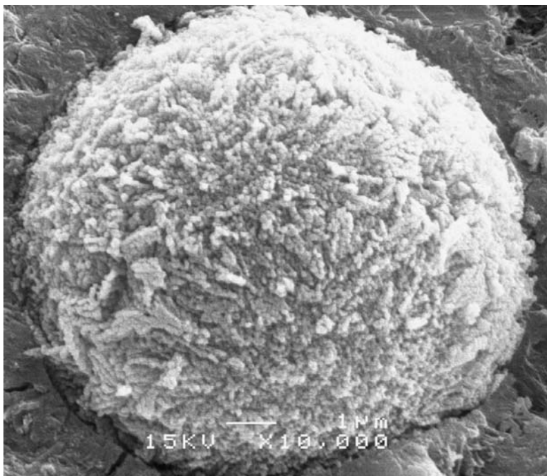
Figure 4-6 Reacted fly ash particle in concrete
