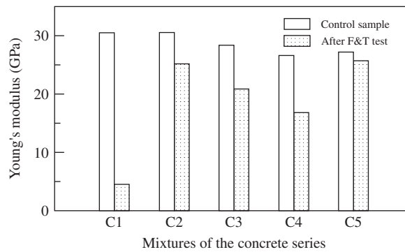
Figure 9-4 Comparison of the elastic modulus of control samples and samples that underwent the freezing and thawing test for the concrete series
