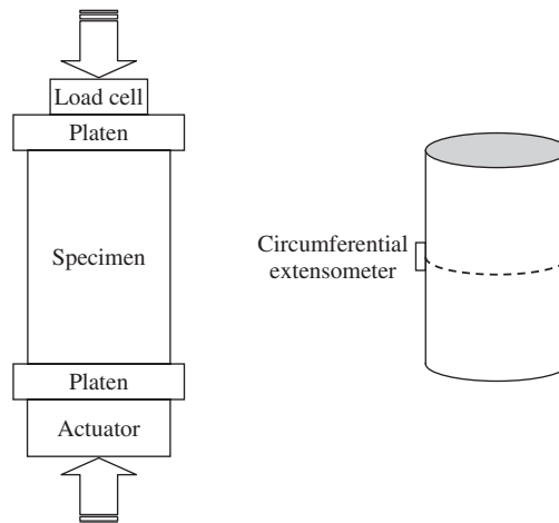
Figure 5-30 Circumferential controlled test setup
