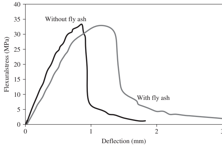
Figure 6-13 Stress–deflection curves of an extruded FRC thin plate
