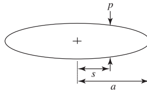
Figure 7-9 A crack under a pair of wedge forces on the right side
