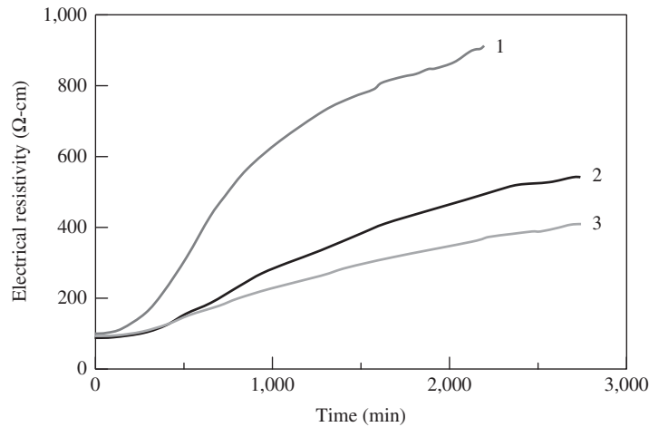
Figure 8-61 Resistivity of cement pastes ( w/c = 1.0, 0.30, 2.0, 0.40, 3.0, 0.50 )
