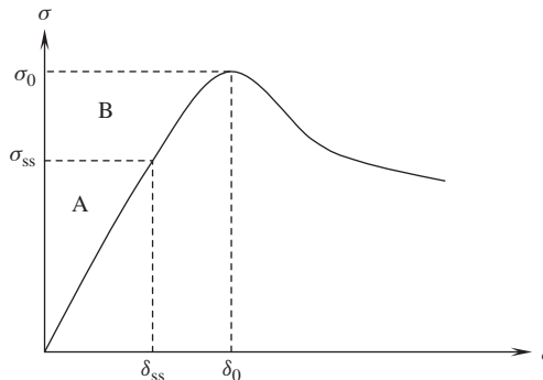
Figure 6-51 Schematic illustration of energy balance concept on a fiber bridging stress-strain curve
