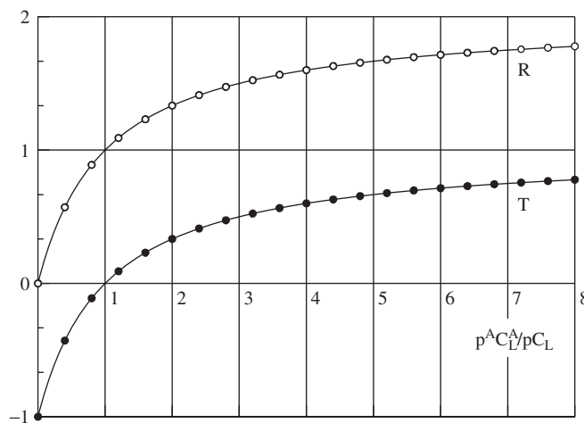
Figure 8-8 The reflection and transmission coefficients vs. acoustic impedance
