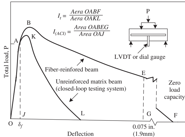
Figure 6-14 Definition of toughness index by ACI
