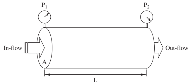
Figure 5-65 Steady-flow permeability test
