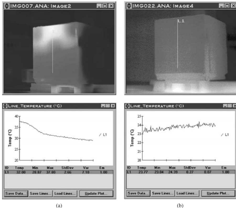
Figure 8-47 Surface temperature distribution of a debonded tile sample with the upper half dry and the lower half filled with water: (a) uniform heating of the inspected face, and (b) after cooling for half an hour
