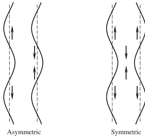
Figure 8-9 Asymmetric and symmetric Lamb waves
