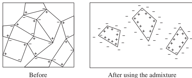
Figure 2-29 Mechanism of water-reducing admixture
