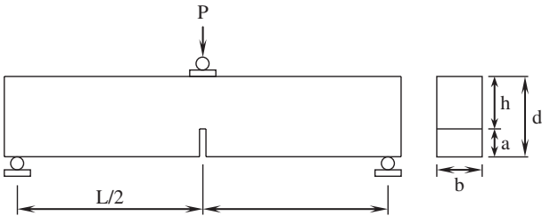
Figure P7-9 Specimen configuration used in the bending tests
