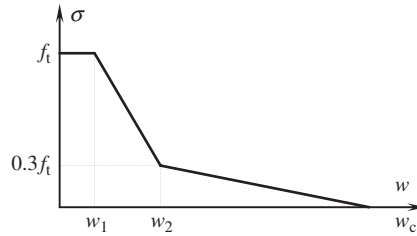
Figure 7-33 Trilinear curve modeling of the closing pressure
