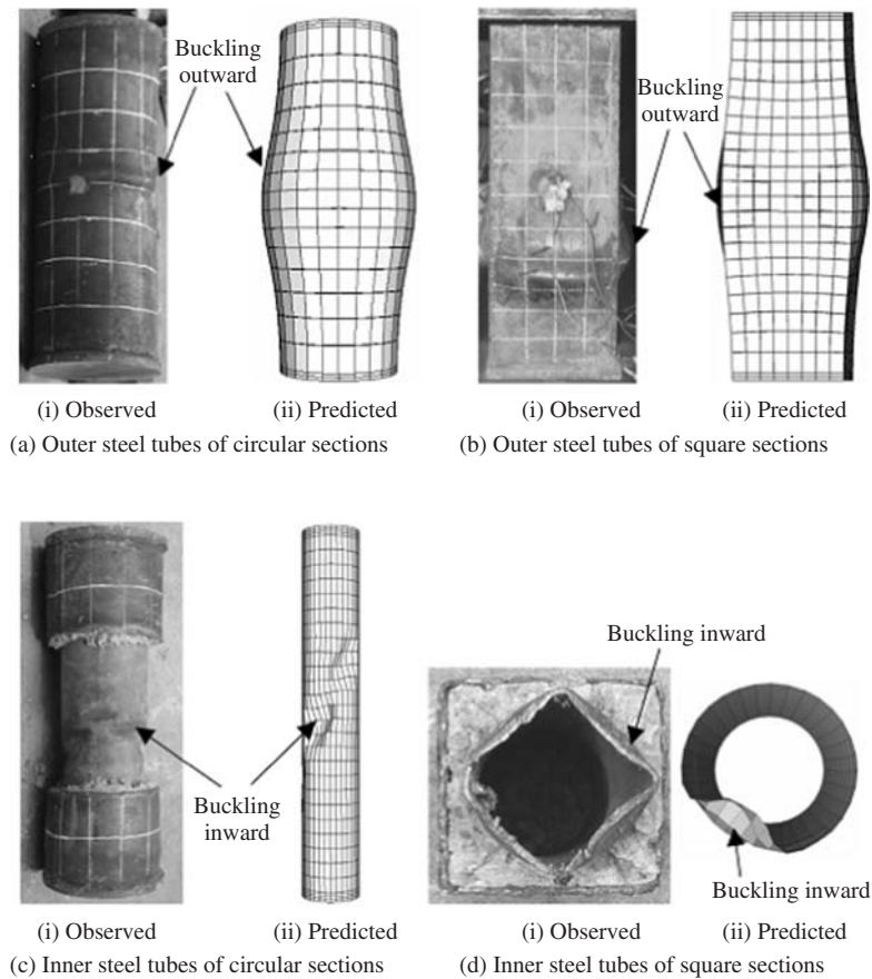
Figure 6-57 Typical failure of hollow CFST
