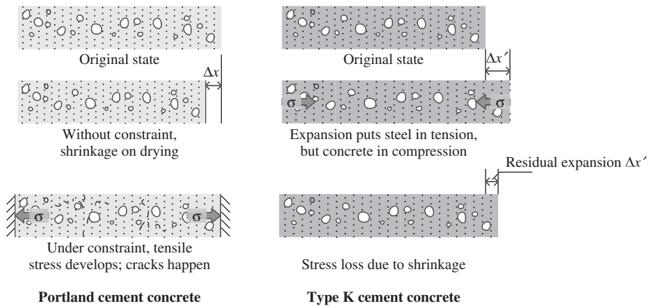
Figure 6-40 Performance of shrinkage-compensating concretes
