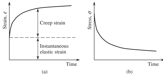
Figure 5-48 The time-dependent behaviors: (a) creep, and (b) relaxation
