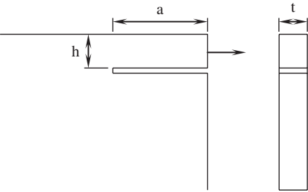
Figure P7-8 A thin plate with an edge crack under plane stress
