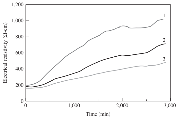
Figure 8-62 Resistivity of mortars (cement/sand = 1, w/c = 1.0, 0.35, 2.0, 0.50, 3.0, 0.70 )
