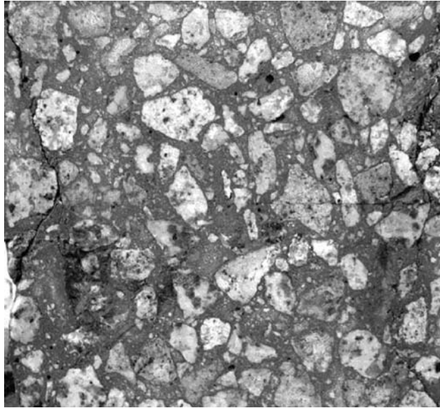
Figure 4-1 Visual level of a concrete's structure (mm scale)
