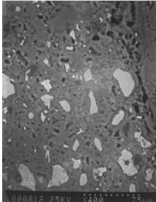
Figure 4-18 Transition zone of high-strength concrete
