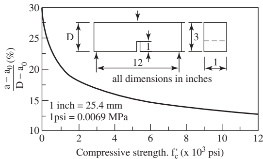
Figure 7-26 Critical crack extension against compressive strength
