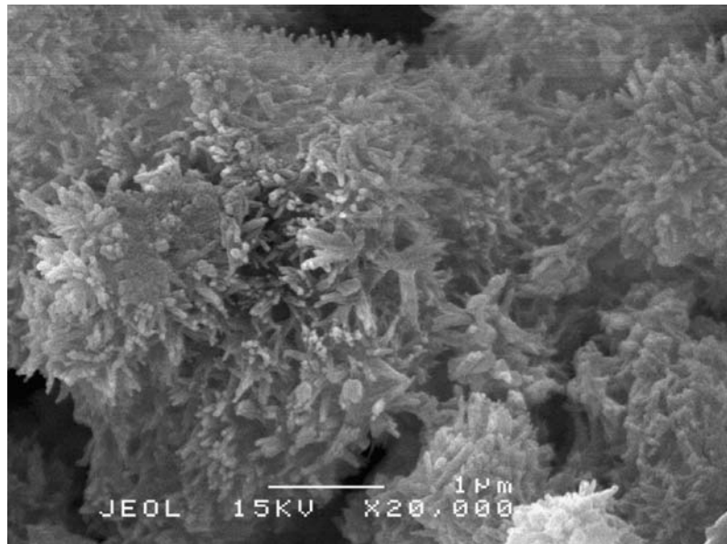
Figure 4-5 Morphology of C-S-H
