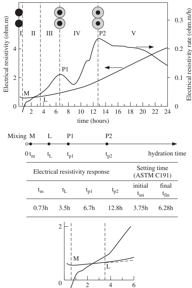
Figure 2-16 Electrical resistivity development and the rate in resistivity of the cement paste during the first 24 h
