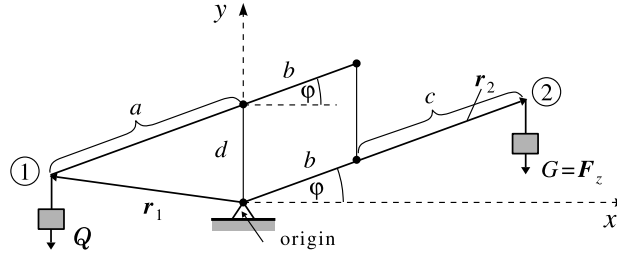
Fig. 15.4. Geometry of the bascule bridge described in the problem
